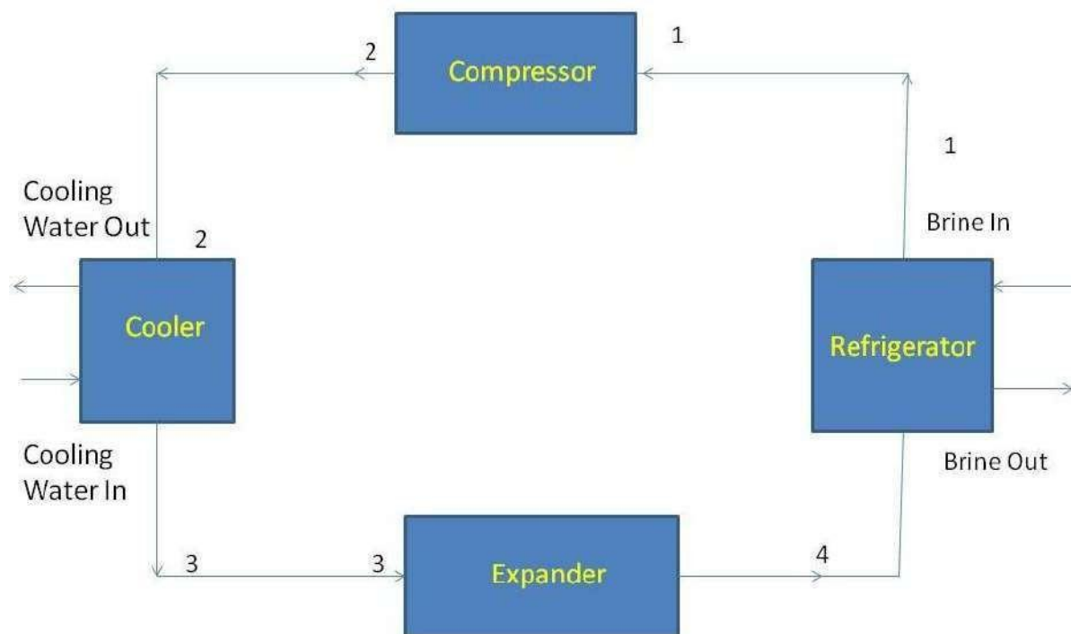
ClosedBellColemanAirCycle
