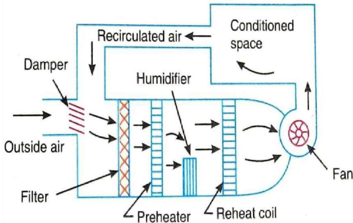
Winter air conditioning system
