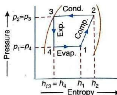
(b) p-h diagram.
