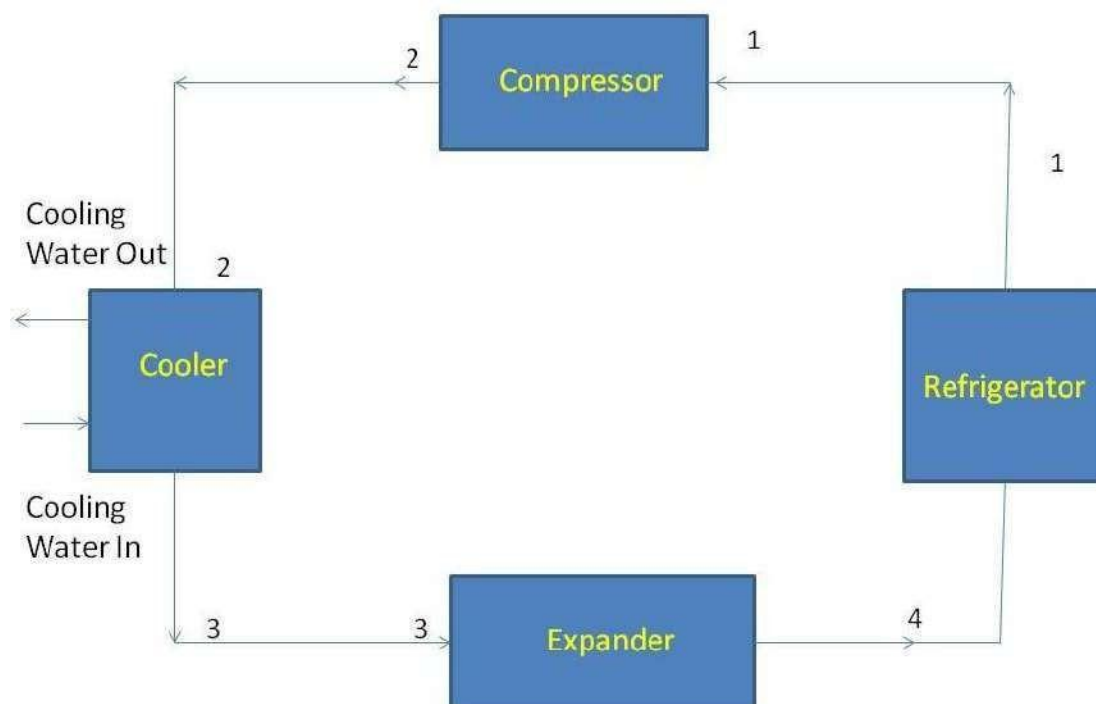
OpenBellColemanAirCycle
