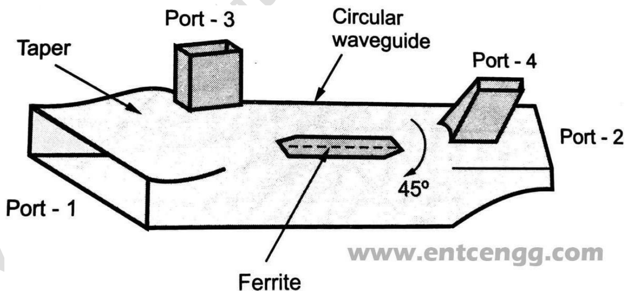
Fig. 2.6.2 Four-port circulator
