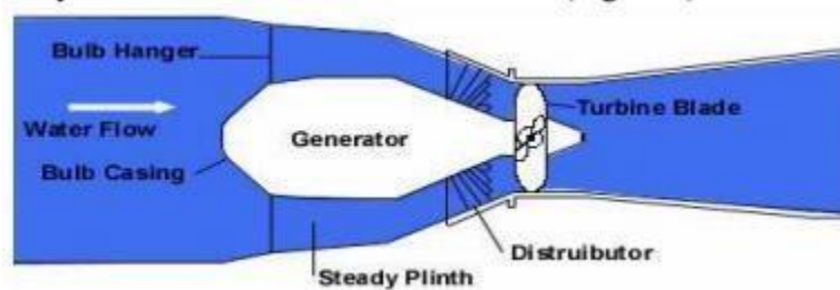
Bulb Turbine
