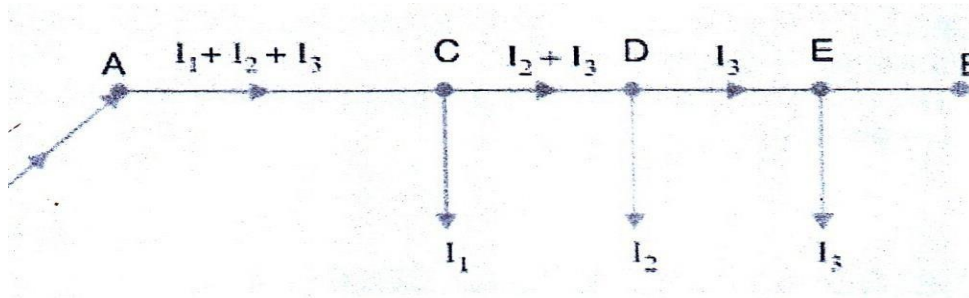
DC Distributor fed at one end
