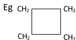
Cyclobutane
