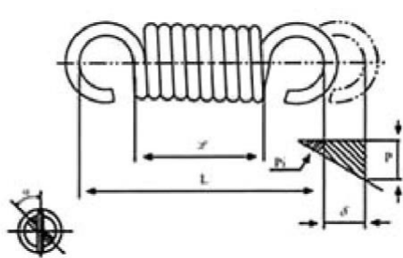
Tension
