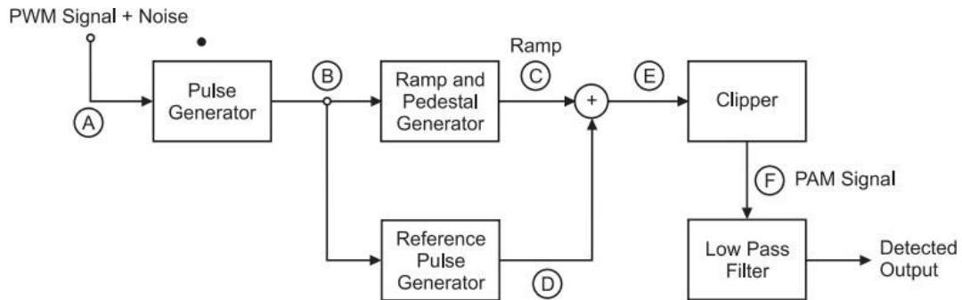
PWM Detector
