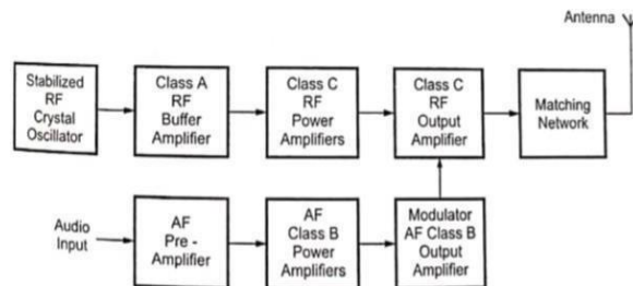
Block Diagram of High Level Modulation
