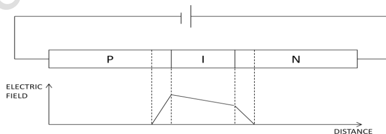
ELECTRIC FIELD DISTRIBUTION UNDER REVERSE BIAS
