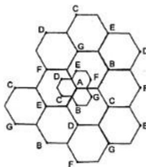
Fig. shows a cell splitting in which a congested cell, divided into smaller micro cells, and the base stations are put up at corners of the cells. The micro-cells are to be added in such a way
