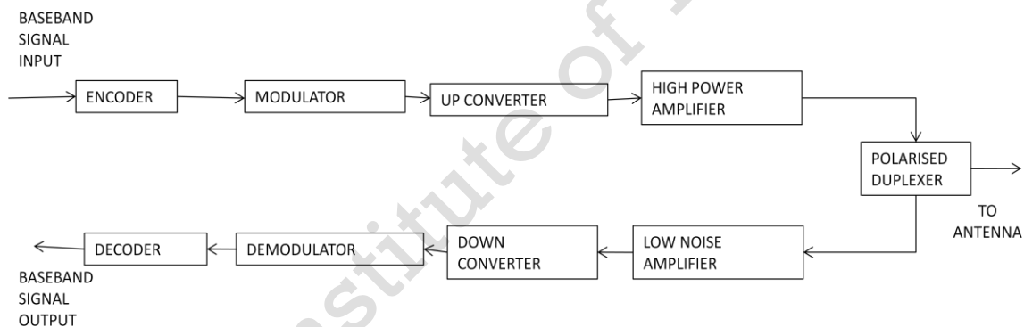
Block diagram of earth station
