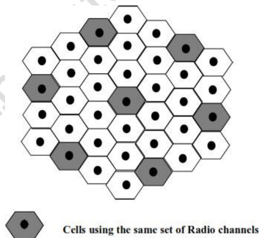
Figure 1. Cellular Network with Frequency Reuse
